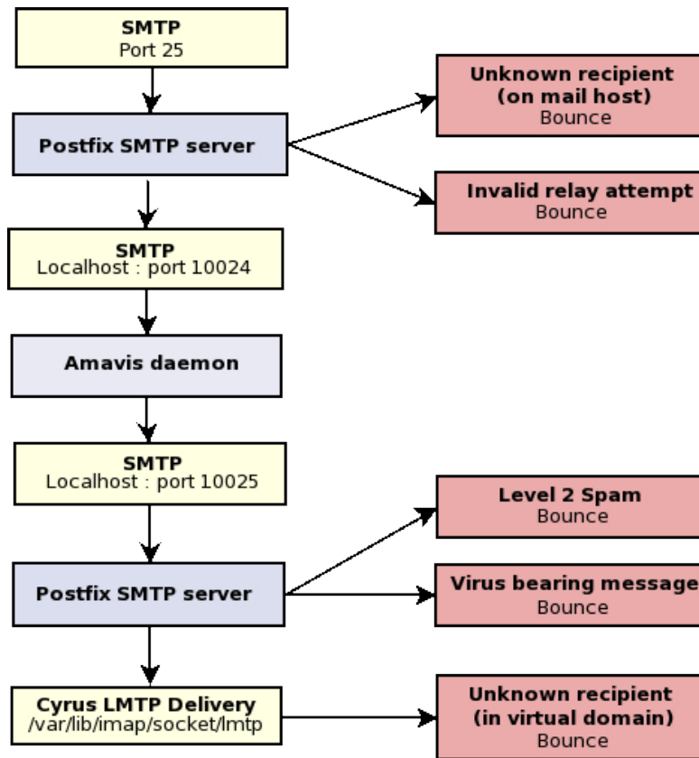
Figure 3: Recipient Verification Using Cyrus IMAP
