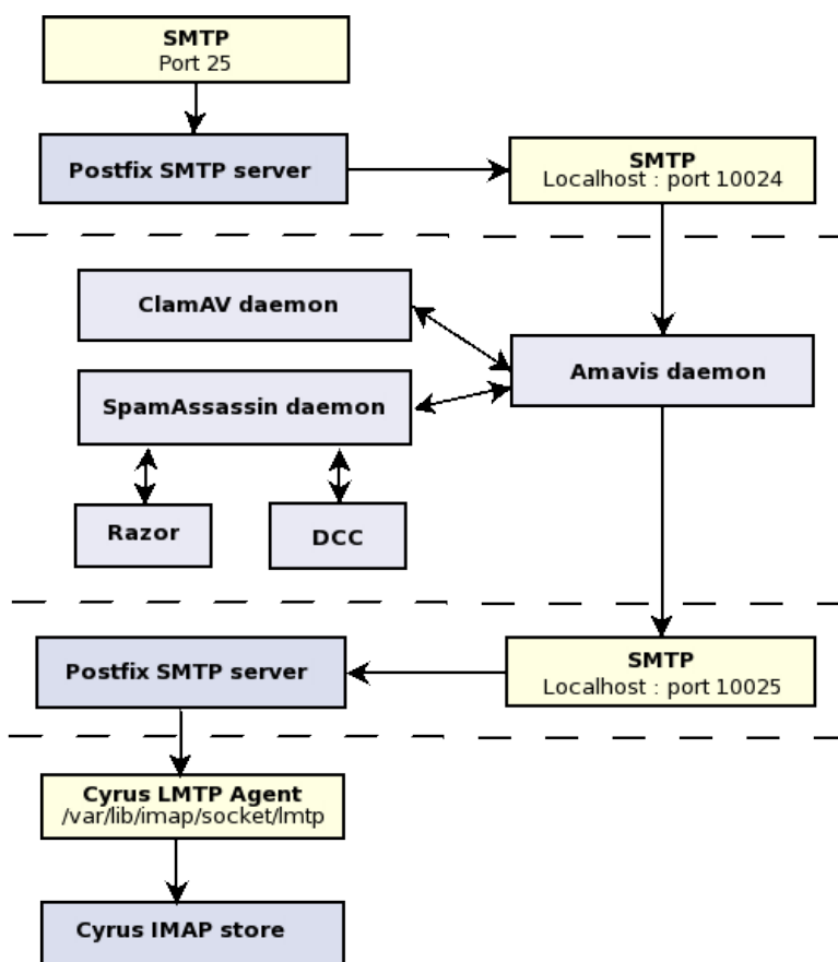
Figure 1: Inbound Mail Routing Diagram
