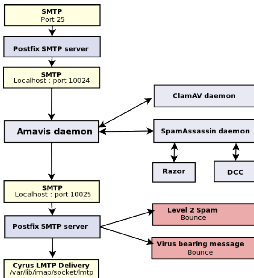
Figure 4: Mail routing with Amavis implementation fleshed out
